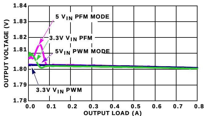
FIGURE 9. V_{OUT} REGULATION vs LOAD 2.25MHz 1.8V _{OUT}
