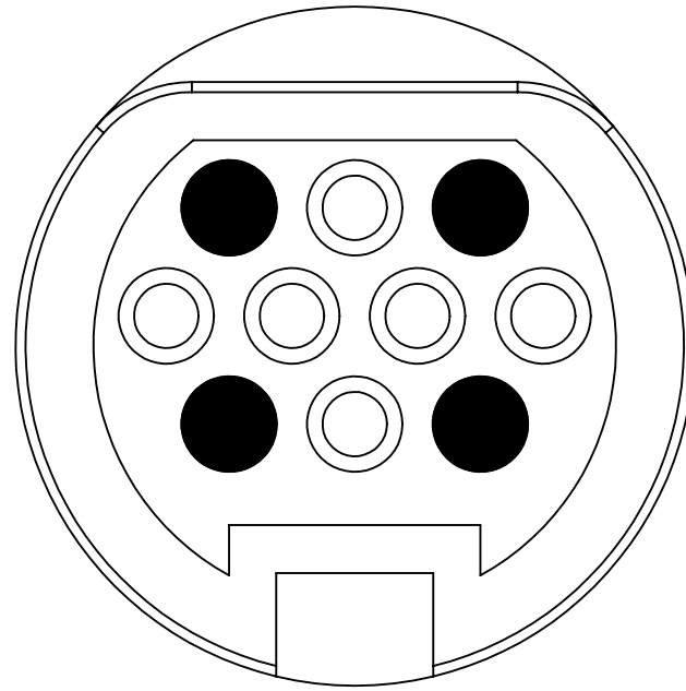
225-A006-04X-XXXX REAR VIEW
