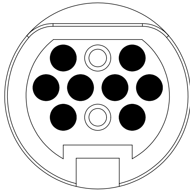
225-A006-08X-XXXX REAR VIEW
