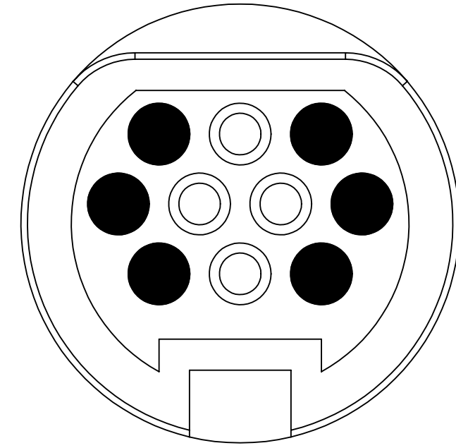
225-A006-06X-XXXX REAR VIEW
